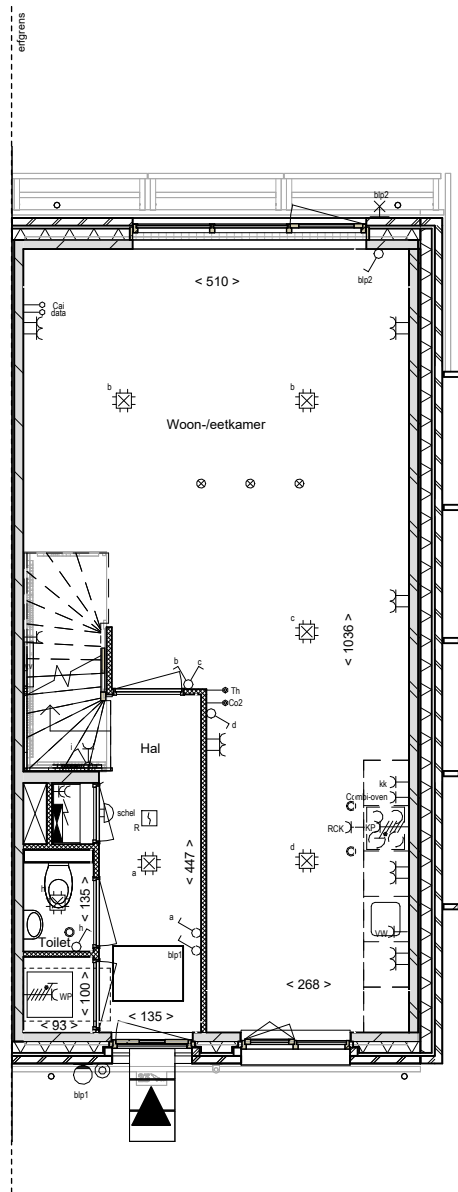
00 begane grond
